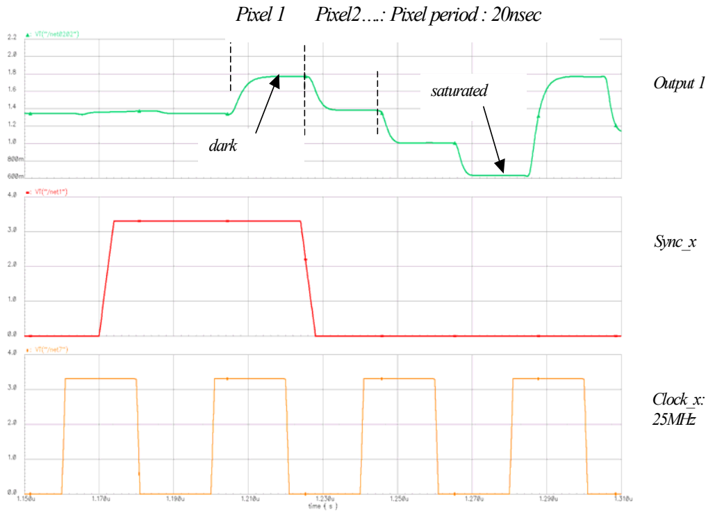
Figure 17: output signal related to Clock_x signal. From bottom to top: Clock_x, Sync_x and output. The output level before the first pixel is the level of the last pixel of previous line.
